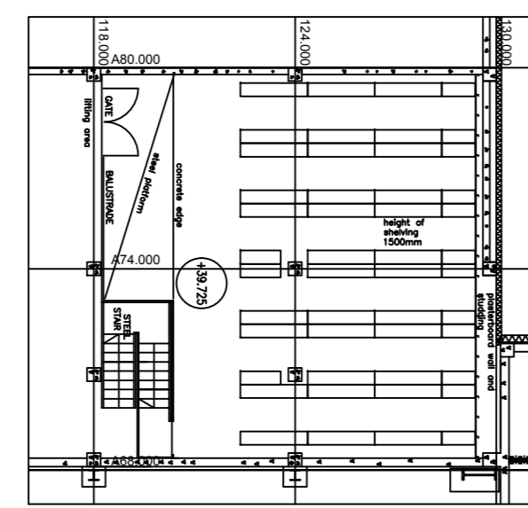
STORE MEZZANINE LEVEL PLAN @ LEVEL +39.725m
